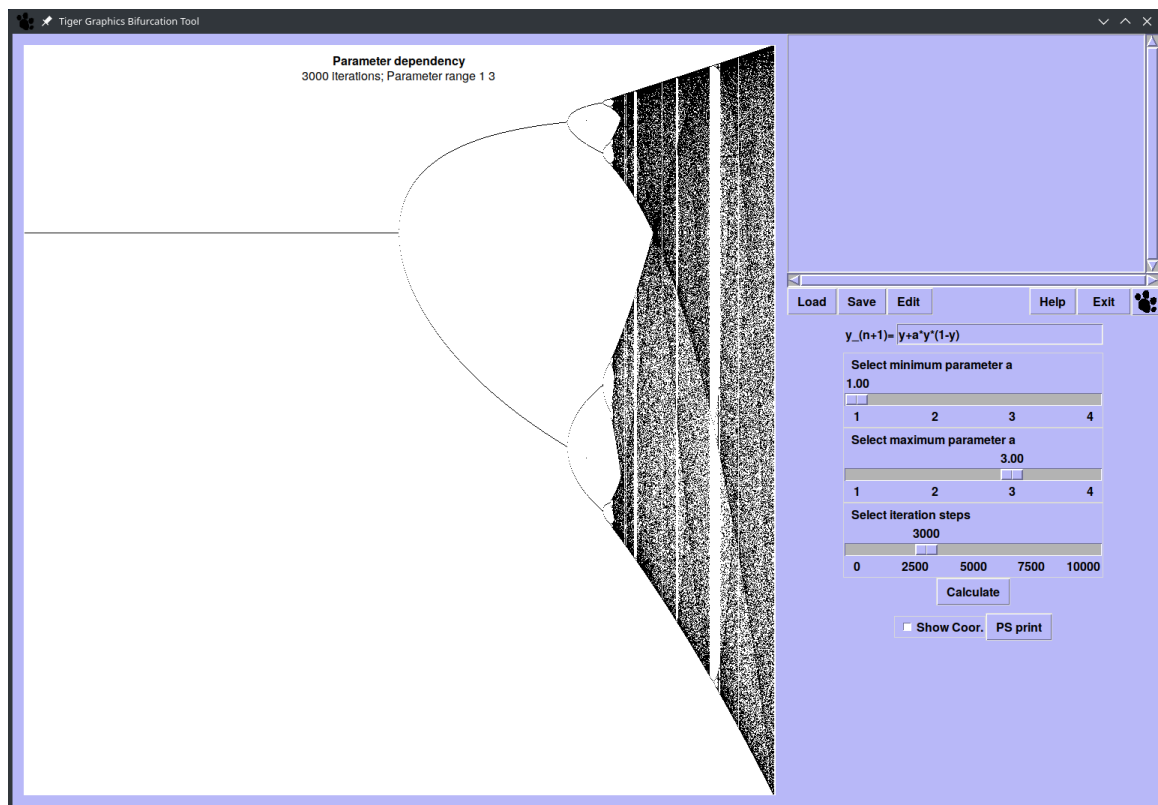
Figure 8.1: The Parabola Widget
