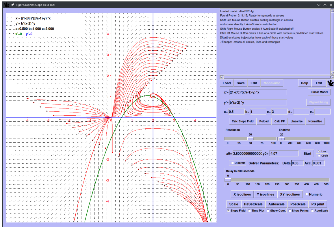
Figure 5.1: The Slope Widget
