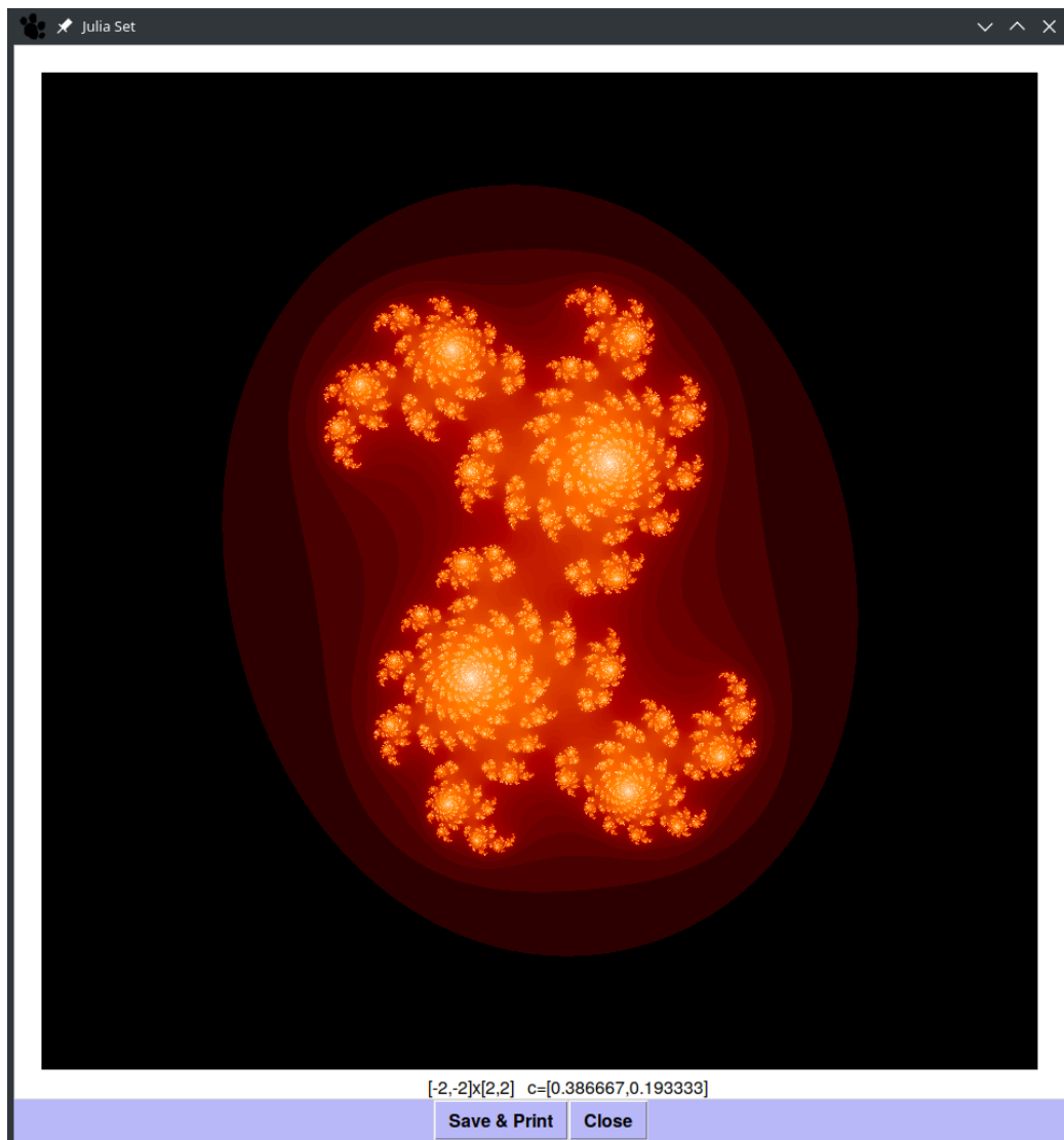
Figure 4.2: A Julia Set
