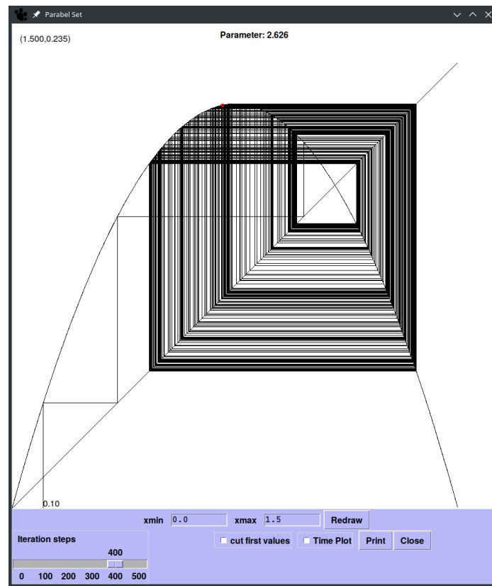
Figure 8.2: A single parabola with its iterations
